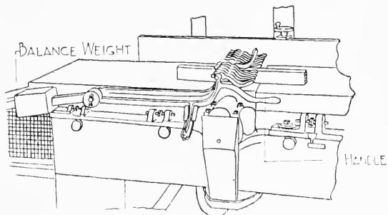
FIG. 150. JOINTER GUARD IN PLACE.
